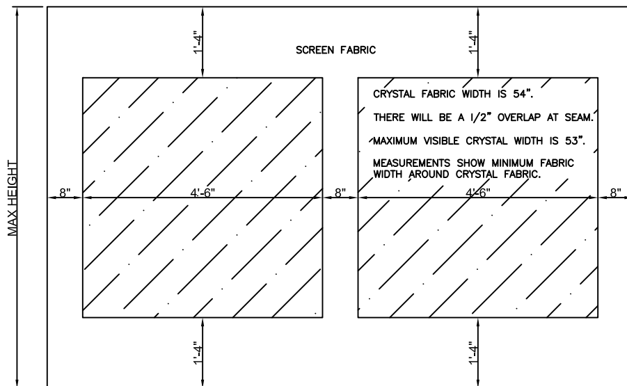
ROLLAC ZIPSHADE 150 SYSTEM SPECIFICATION WITH CRYSTAL FABRIC INSERTS FOR VISIBILITY.
